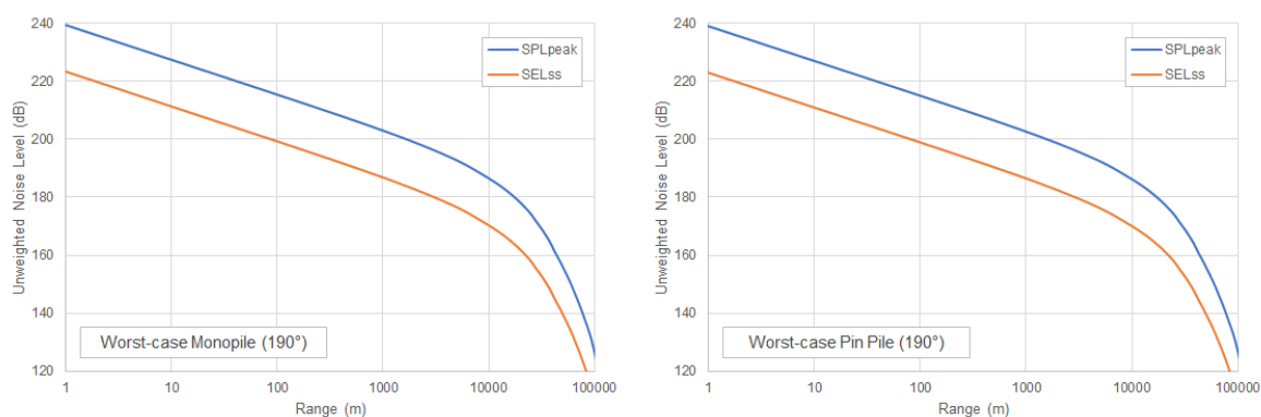
Figure 5-10 Level against range plots showing the unweighted SPL_{peak} and SEL_{ss} noise levels from the worst-case locations for monopiles and pin piles at EA1N for a deep transect ( 190^\circ )
