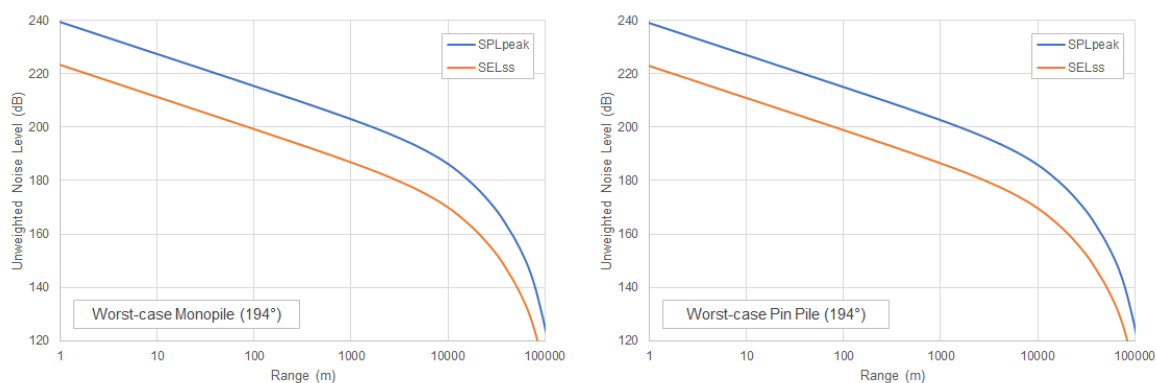
Figure 5-9 Level against range plots showing the unweighted SPL_{peak} and SEL_{ss} noise levels from the worst-case locations for monopiles and pin piles at EA2 for a deep transect ( 194^\circ )
