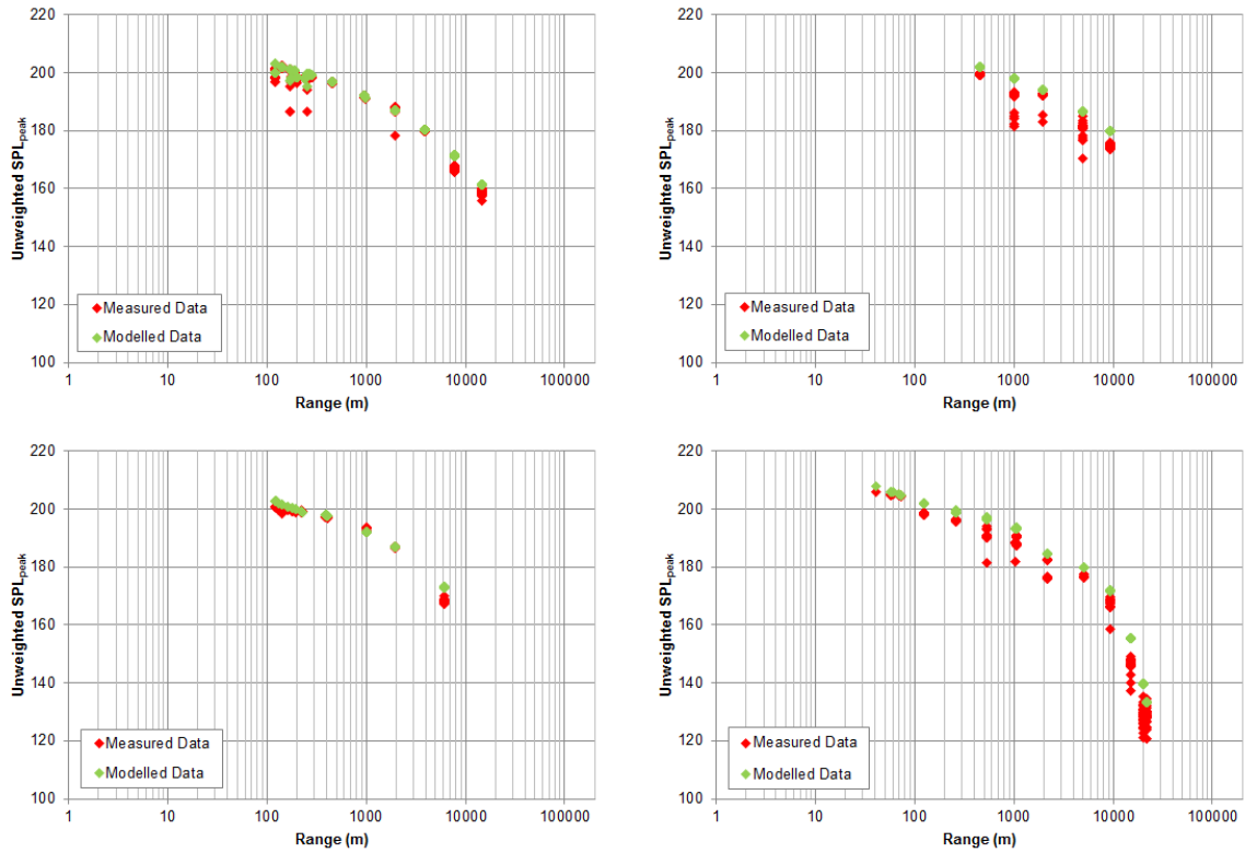
Figure 4-3 Comparison between example measured data (red points) and modelled data using INSPIRE version 4.0 (green points)
