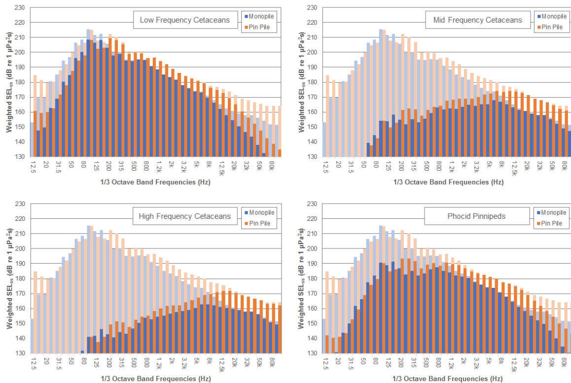
Figure 5-11 Filtered noise inputs for monopiles and pin piles using the NMFS (2018) filters. The lighter coloured bars show the unweighted third octave levels
